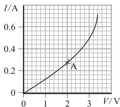
Thermistor
